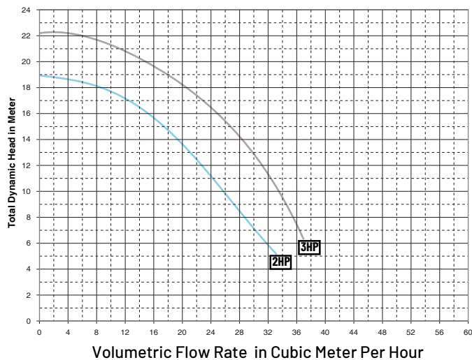
Pump Performance Curves (50hz)
