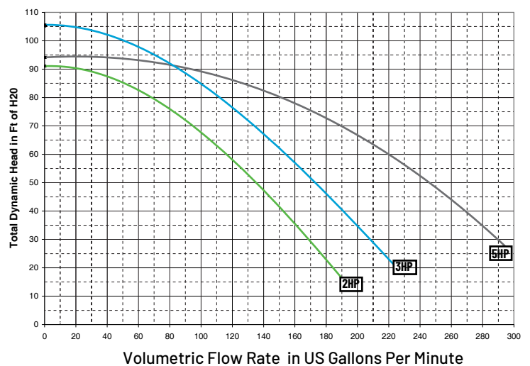
Pump Performance Curves (60hz)
