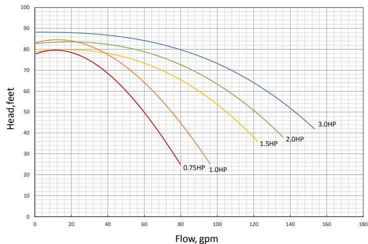
60Hz Performance Curve
