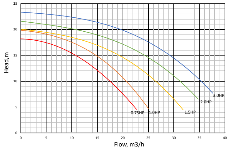
60Hz Performance Curve
