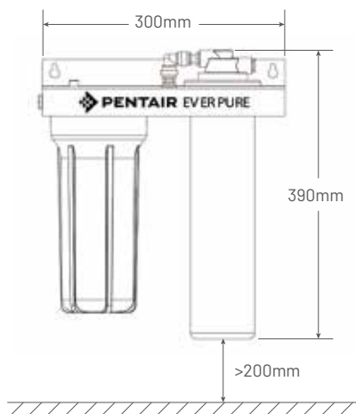
Everpure Combo-4FCS-CN Commercial Water Purifier
